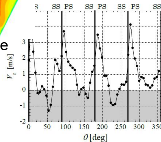
Fig.8 Outlet velocity distribution of pump
