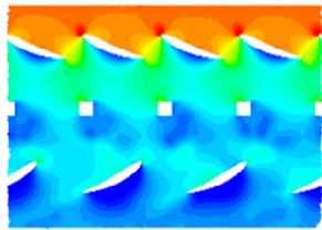
Fig.3 Blade-to-blade flow
