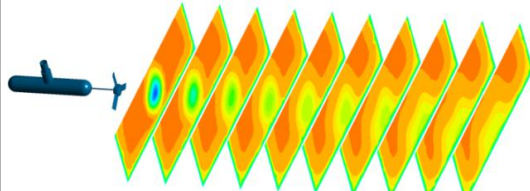
Fig.5 Wake from propeller turbine
