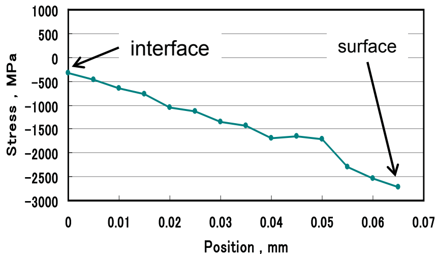
Fig.1. Internal stress of Cu layers in AIN/Cu multi-layer film
