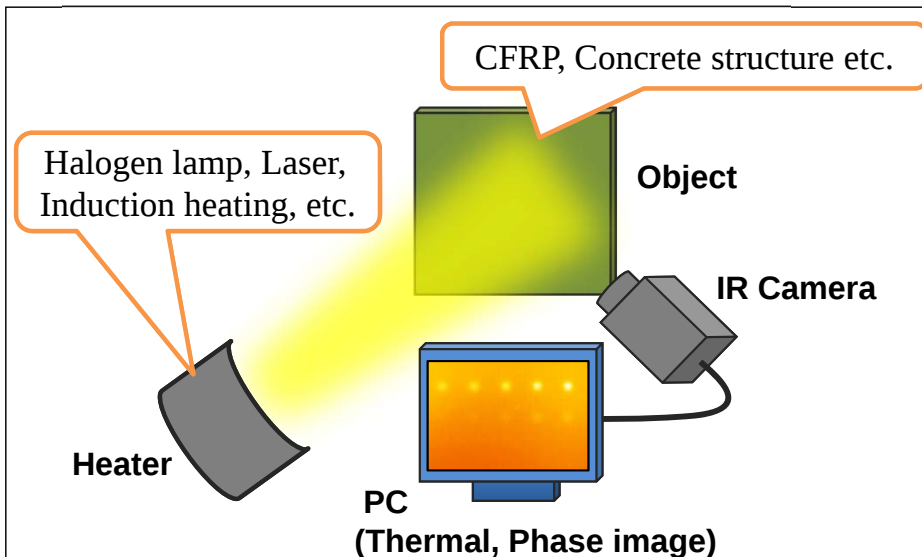
Fig. 1 Schematic illustration of infrared thermographic testing.
