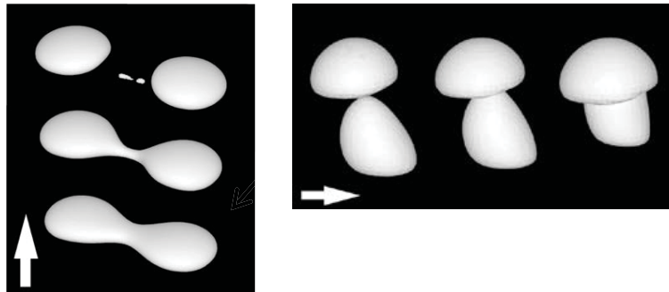
Fig. 2 Complex motion of bubble and drop. Left: drop breakup Right: bubble merging
