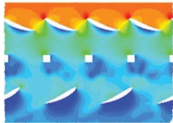
Fig.3 Blade-to-blade flow
