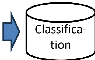
2. Insect classification
