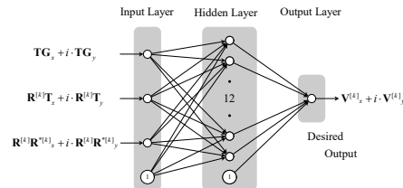
Complex-valued NN
