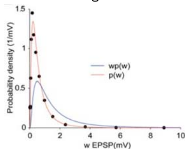
Fig. 2 Heavy tail distribution
