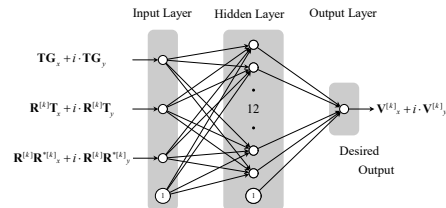
Complex-valued NN
