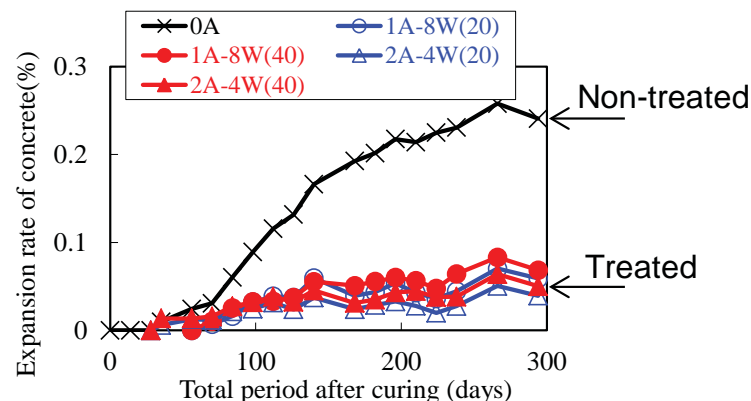
Fig.3 Suppression of concrete expansion due to applying electric current
