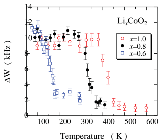
Temperature dependence of {}^7\text{Li} -NMR line widths in Li_xCoO_2 .
