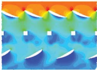
Fig.3 Blade-to-blade flow
