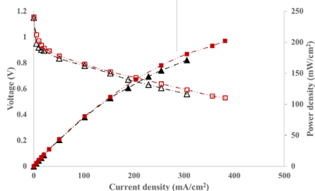
IV curves of SOFC cell at 800 C.
