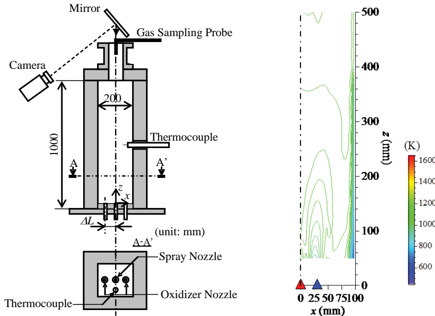
Fig. 1 HiTAC furnace.
