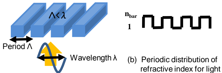
(a) Schematic diagram Fig.1 Sub-wavelength grating structure
