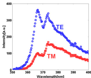
Fig.4 Emission spectra from UV-LED
