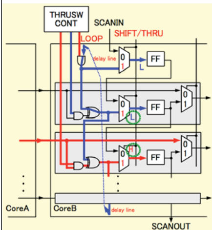
Fig.2 Boundary scan with TDC
