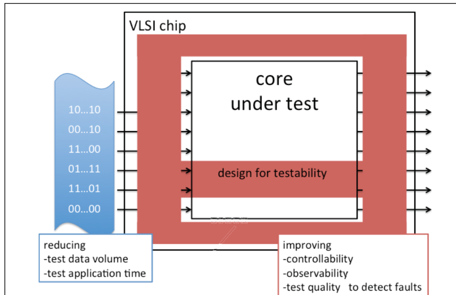
Fig.1 overview of design for testability
