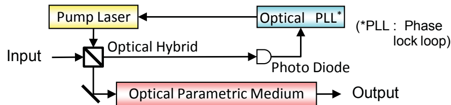
(b) Basic configuration of PSA
