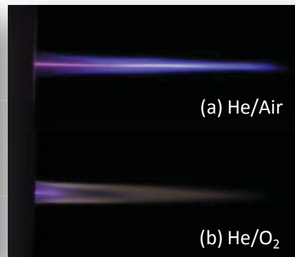
Fig. 3 SGF Plasma jet
