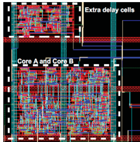
Fig.3 layout of an experimental chip
