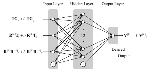
Complex-valued NN
