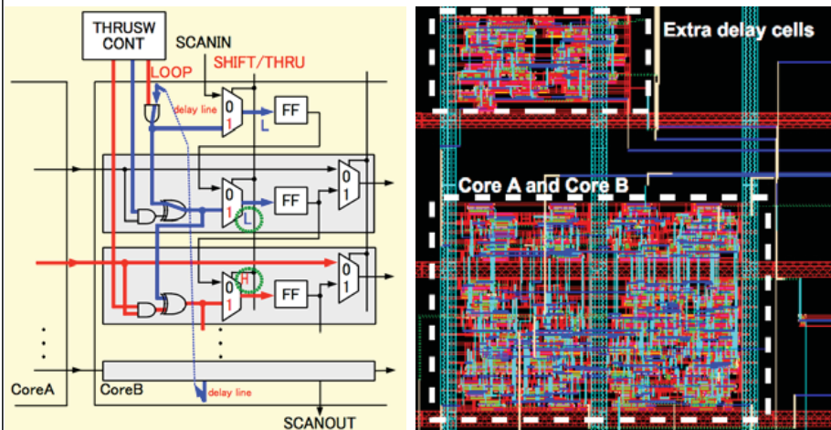
Fig.2 Boundary scan with TDC
