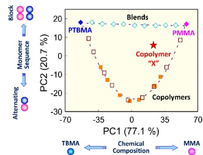
Fig. 2 Principal component score plots showing chemical composition and monomer sequence distribution in methacrylate copolymers.
